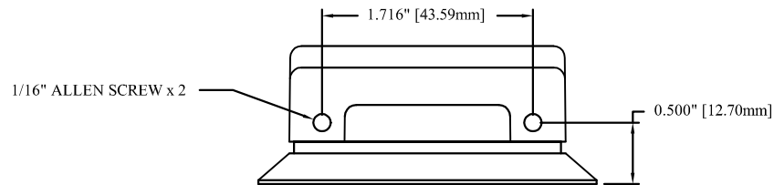
End View:
