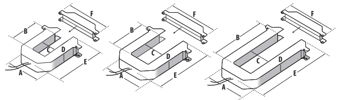
H681x-5A Split-core
